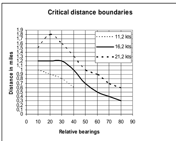
Fig. 5. Critical distance boundaries
