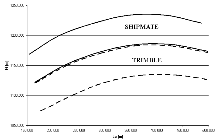
Fig. 5. The enlarged part of Figure 4- the outer curves represent mean trajectories of given receivers and the inner curves represent the trajectories of mean values with constraints
