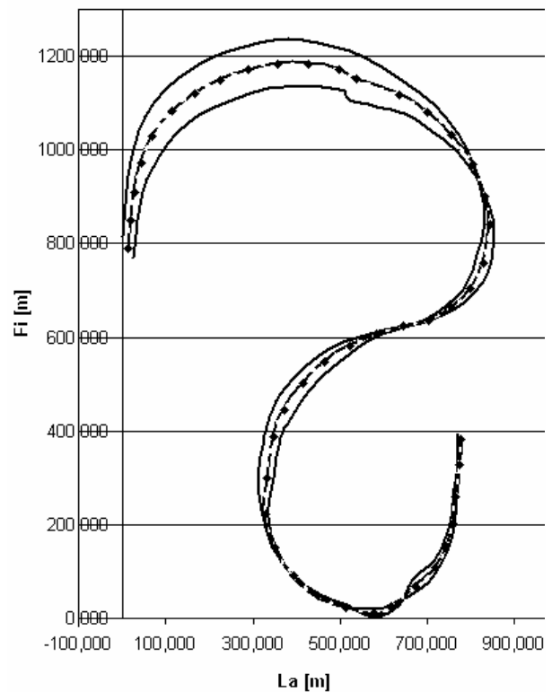
Fig. 4. Estimation with constraints with the use of true GPS measurements - circulating vessel ('eight'- shaped curve)
