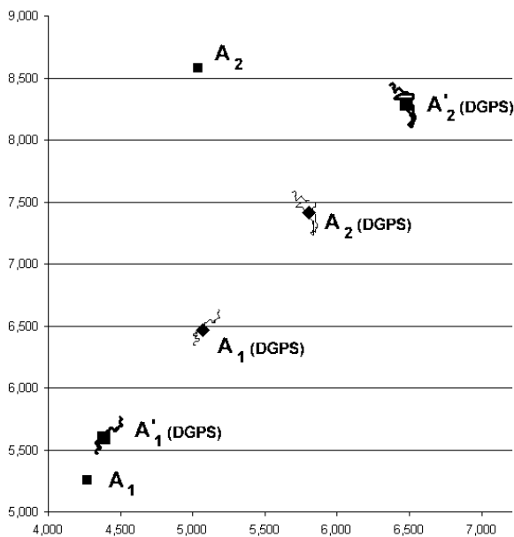
Fig. 3. Estimation with constraints with the use of true GPS/DGPS measurements
