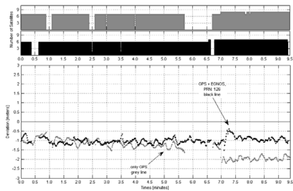
Fig. 1. Septentrio X Coordinate Deviation, 15 Deg. Mask
