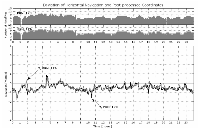
Fig. 12. PRN 120 vs. 126, Y-Coordinate
