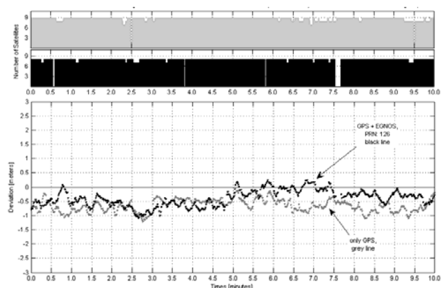
Fig. 6. Septentrio X Coordinate Deviation, 0 Deg. Mask
