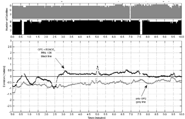
Fig. 5. CSI Y Coordinate Deviation, 0 Deg. Mask
