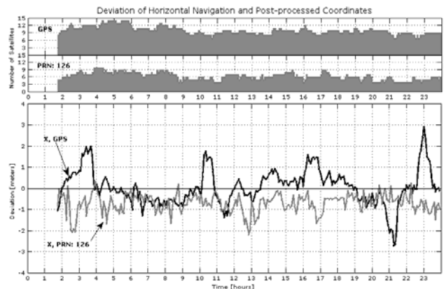
Fig. 8. GPS vs. PRN126, X-Coordinate
