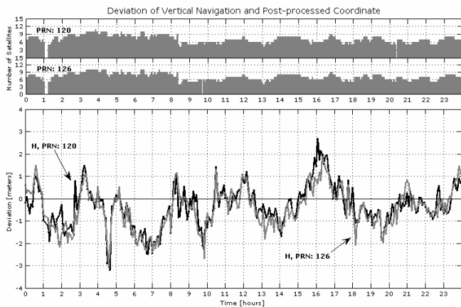
Fig. 13. PRN 120 vs. 126, Height
