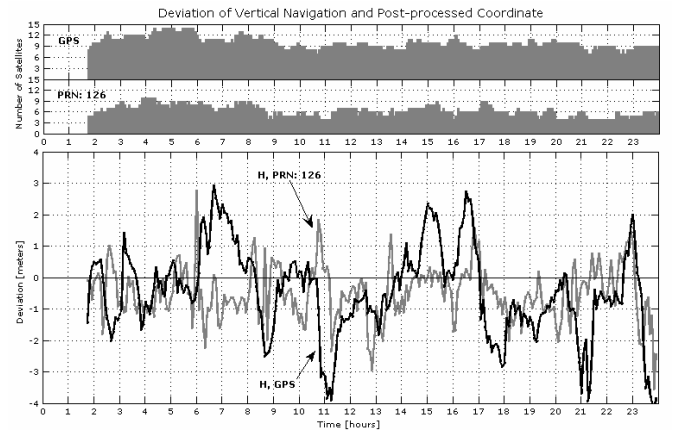
Fig. 10. GPS vs. PRN126, Height
