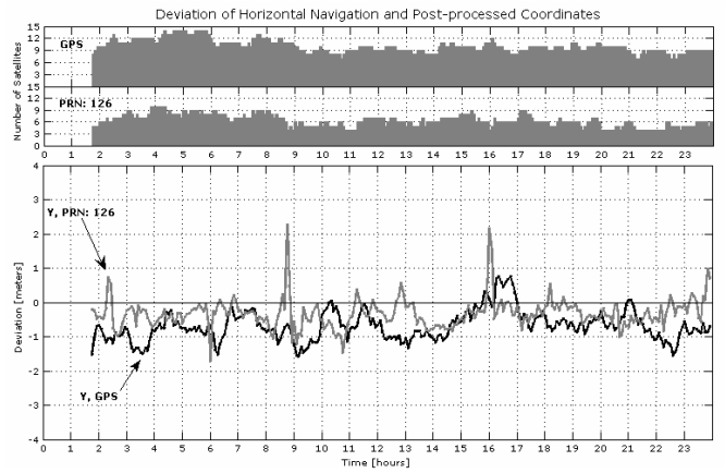
Fig. 9. GPS vs. PRN126, Y-Coordinate
