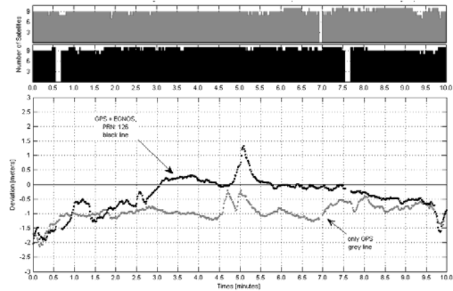
Fig. 4. CSI X Coordinate Deviation, 0 Deg. Mask
