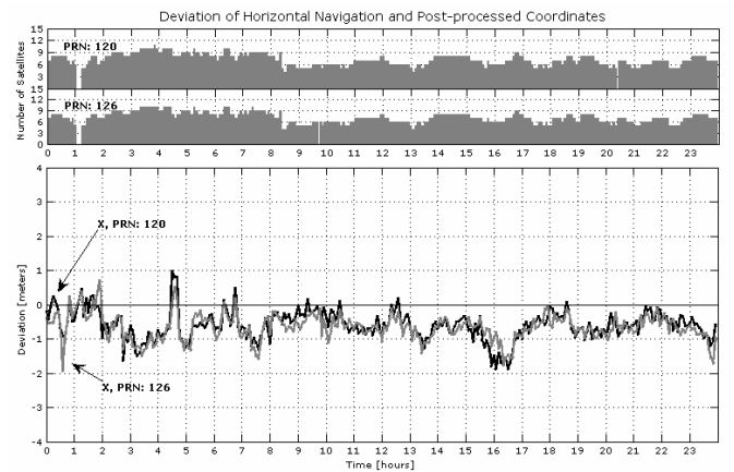
Fig. 11. PRN 120 vs. 126, X-Coordinate
