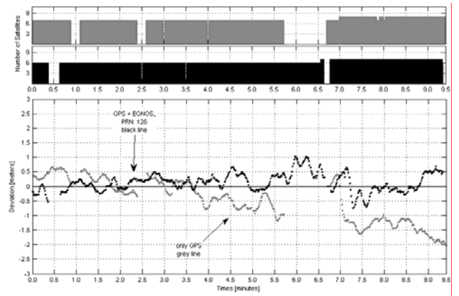
Fig. 3. Septentrio Height Deviation, 15 Deg. Mask
