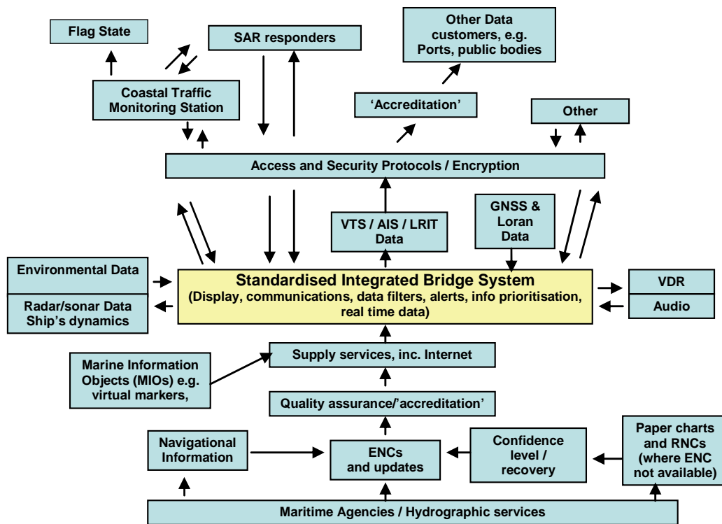
Fig. 2. E-Navigation system architecture [NAV 53/13/...]
