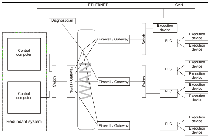
Fig. 1. Construction of a system with devices protecting against access of unauthorized persons
