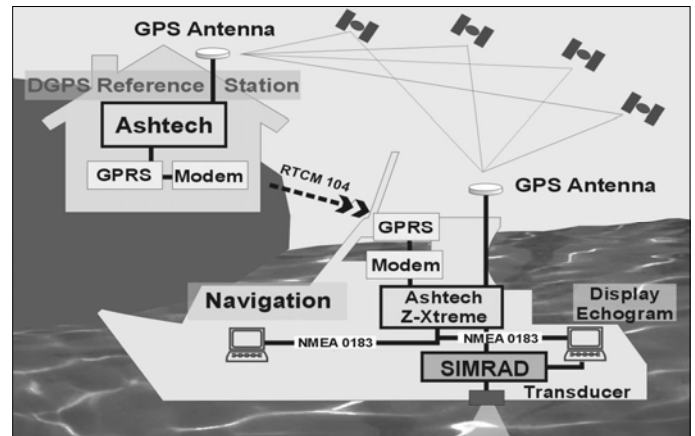
Fig. 2. Integrated Bathymetric System
