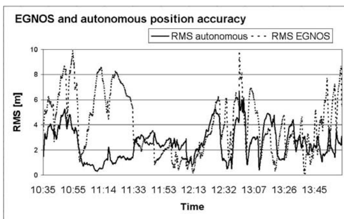
Fig. 7. Dynamic GPS autonomous and EGNOS corrected position accuracy
