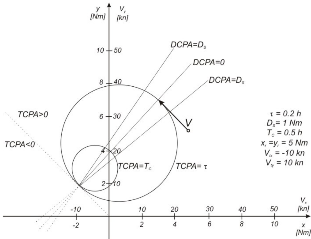
Fig. 1. The Collision Threat Parameters Areas method
