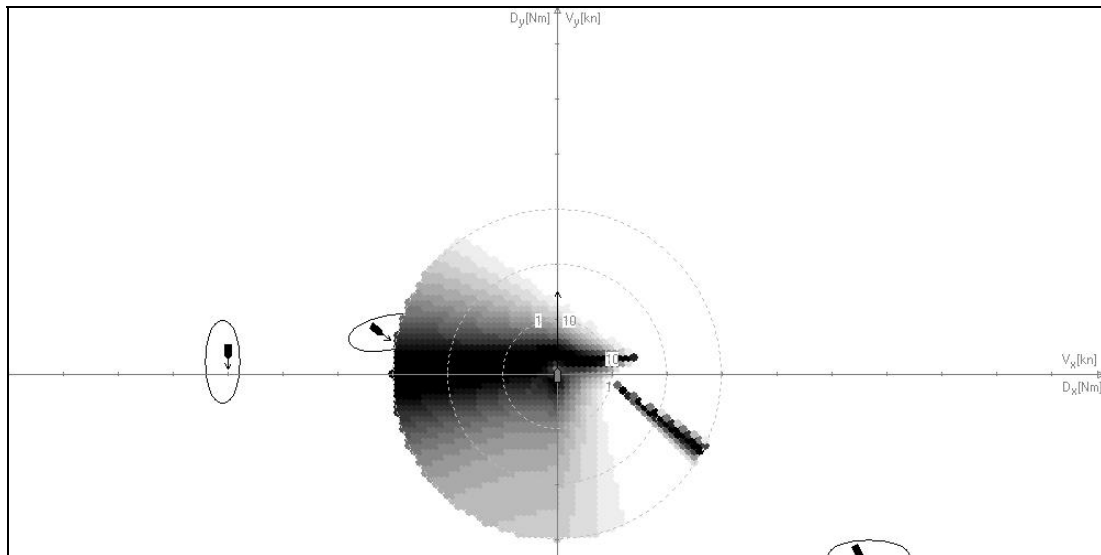
Fig. 7. The FCTPA for the given scenario for the time t = 11 min. (before target 3 has altered its course)
