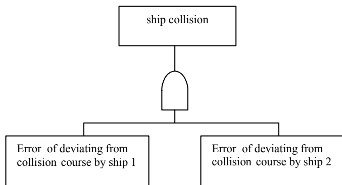
Fig. 4. Fault tree of ship collisions
