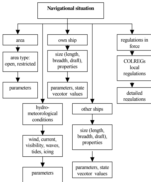
Fig. 1. Model of ship encounter situations
