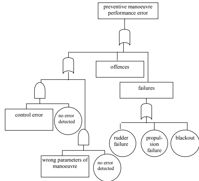
Fig. 6. Fault tree of a collision situation identification error
